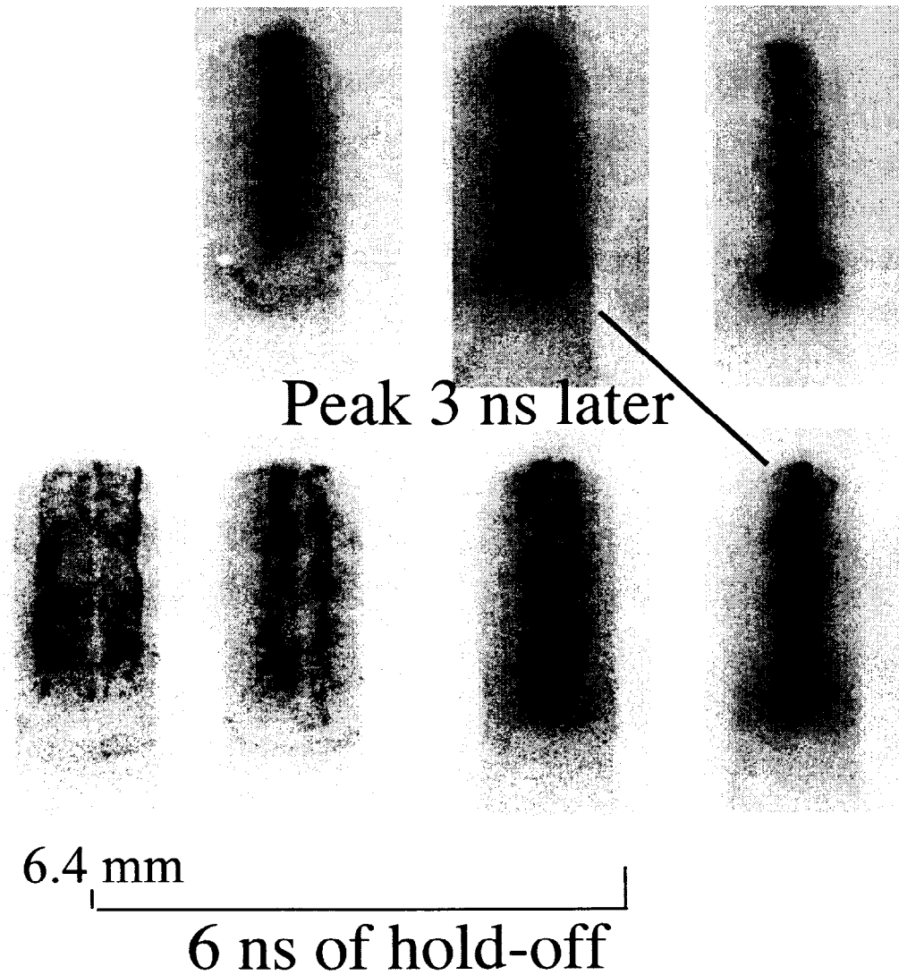
Fig. 3. Soft x-ray (200-280 eV) framing camera images of pinches without (top) and with (bottom) the central foam. The time in ns, with respect to figure 1, is shown above the images.
