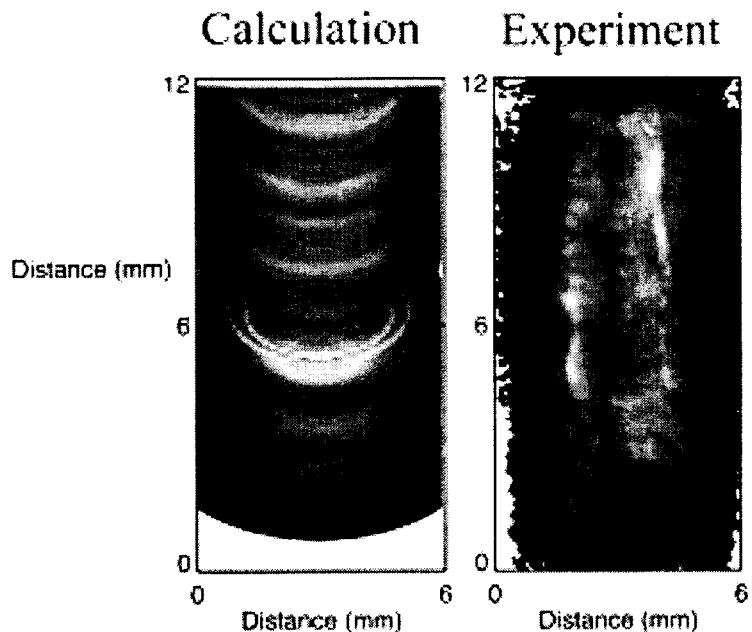
Fig. 4. Simulated soft x-ray framing-camera image and data at 85 ns.
